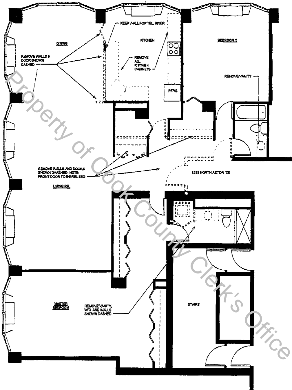
① EXISTING FLOOR PLAN 1/4" = 1'-0"
